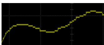
Vectors
